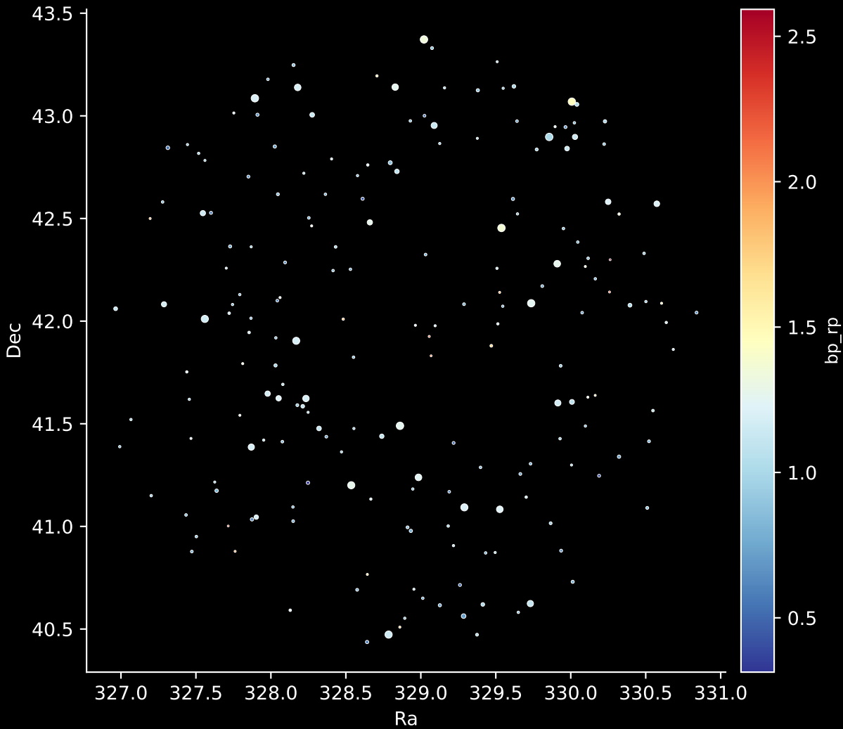
APOGEE DR17 Field: [069+57_MGA] Stars: 198
