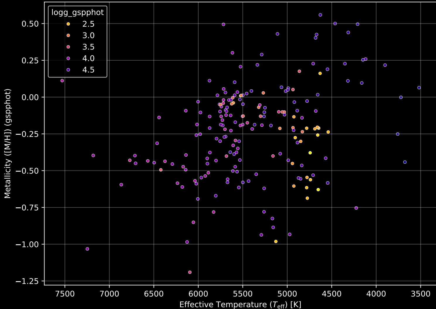
APOGEE DR17 Field: [069+57_MGA] Stellar Population Parameters (n= 198)
