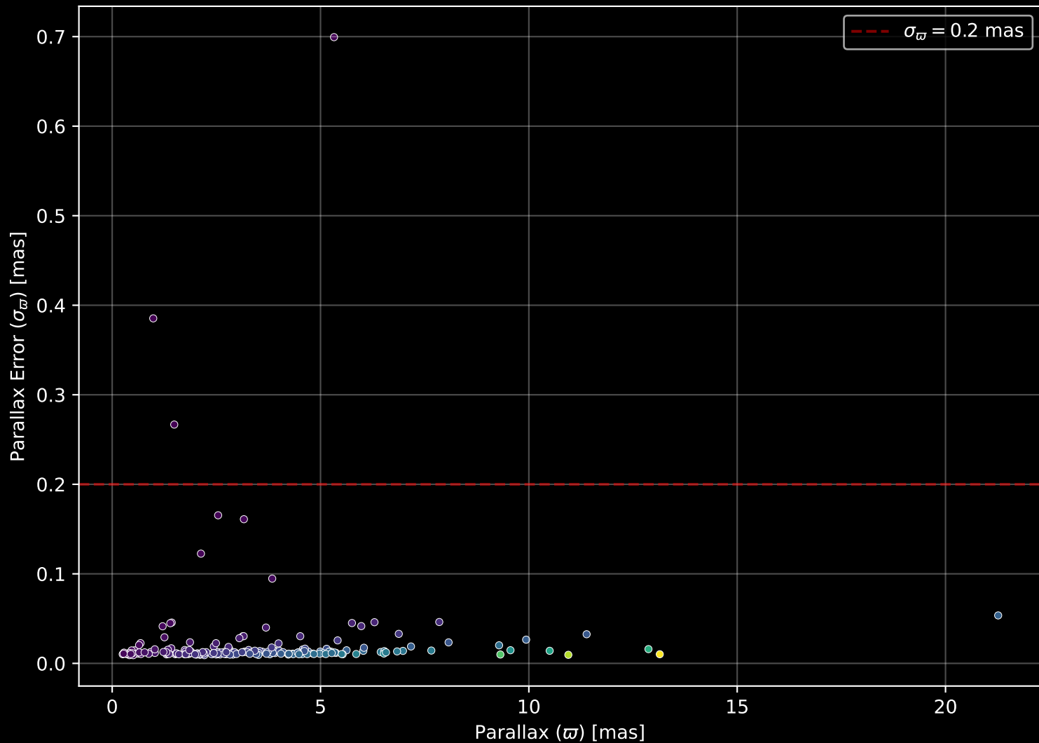
APOGEE DR17 Field: [069+57_MGA] Parallax Quality (n= 198)
