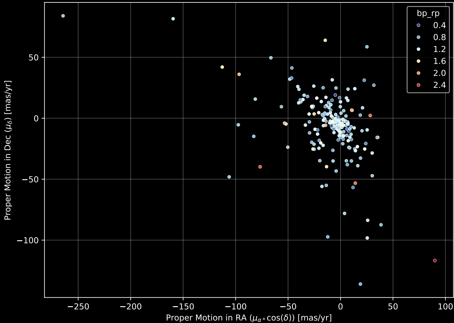
APOGEE DR17 Field: [069+57_MGA] Proper Motion Diagram (n= 198)
