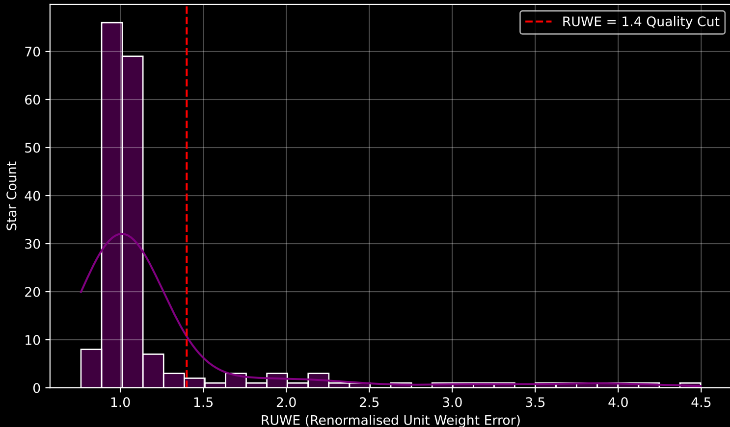
GAPOGEE DR17 Field [069+57_MGA] RUWE Distribution (n= 191)
