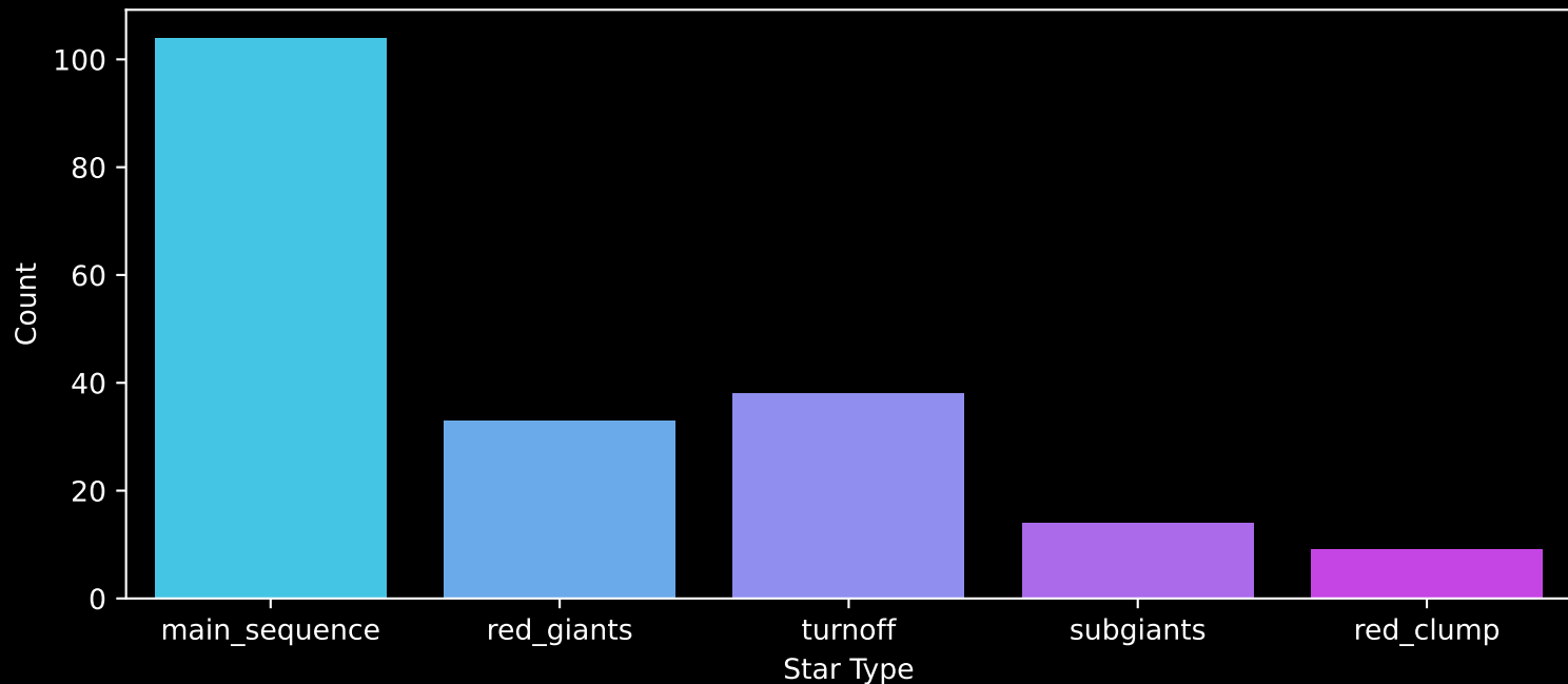
APOGEE DR17 Field: [069+57_MGA] Count plot of Star Type
