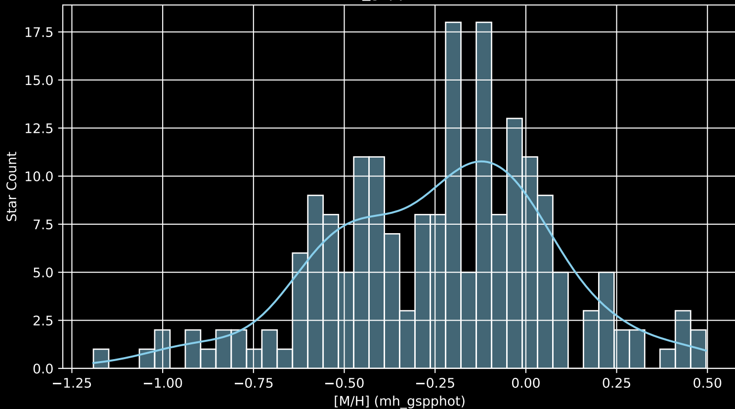
APOGEE DR17 Field: [069+57_MGA [M/H] (mh_gspphot) (n= 196)
